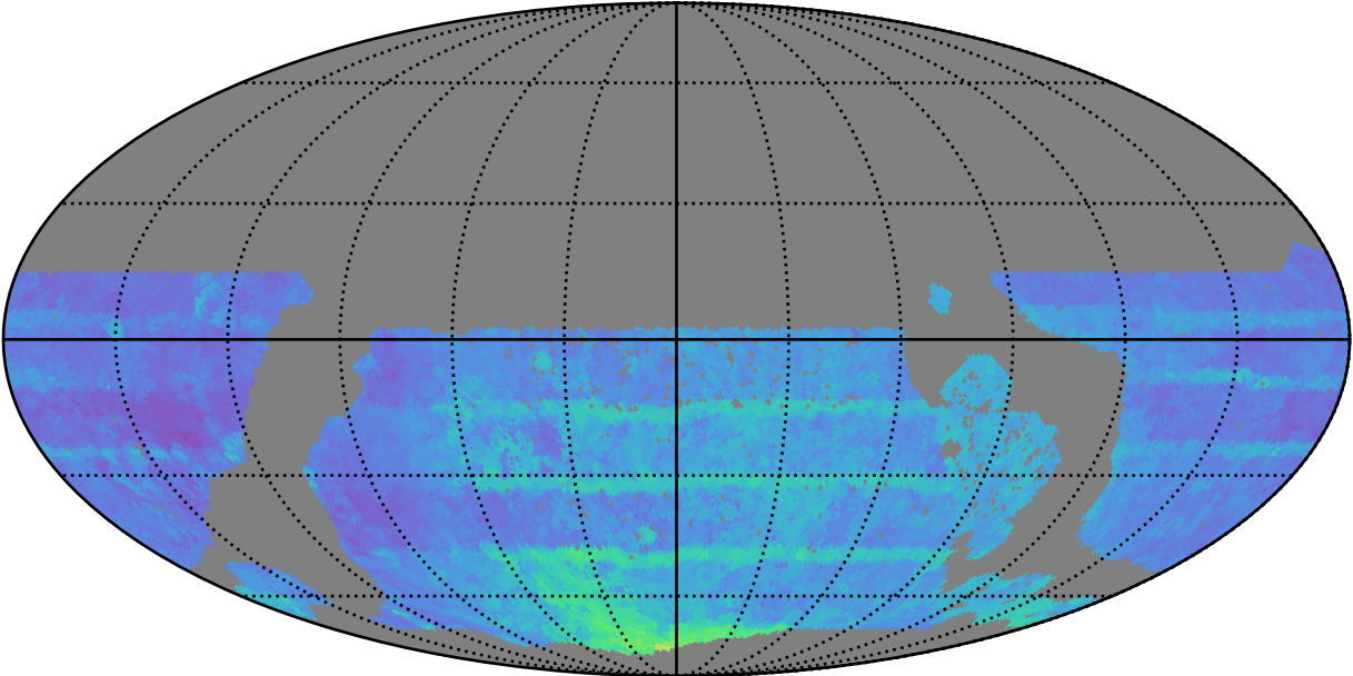
too_combined_s0.8_v3.4_10yrs WFD all bands: 80thPercentile Season Length
