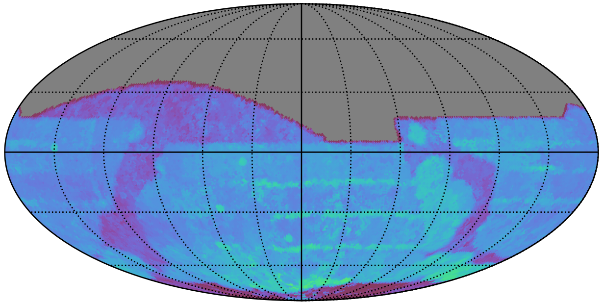
too_combined_s0.8_v3.4_10yrs All sky r band: 80thPercentile Season Length
