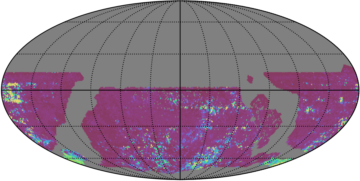
too_combined_s0.8_v3.4_10yrs WFD z band: 75th Percentile Intranight Timespan
