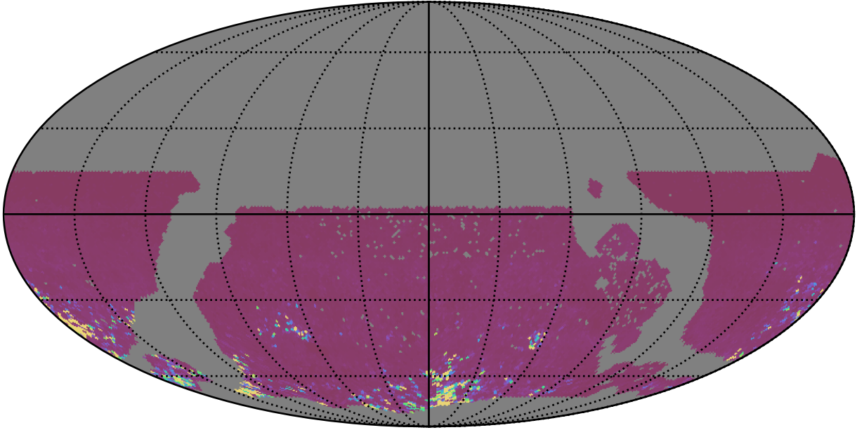
too_combined_s0.8_v3.4_10yrs WFD gr bands: 75th Percentile Intranight Timespan
