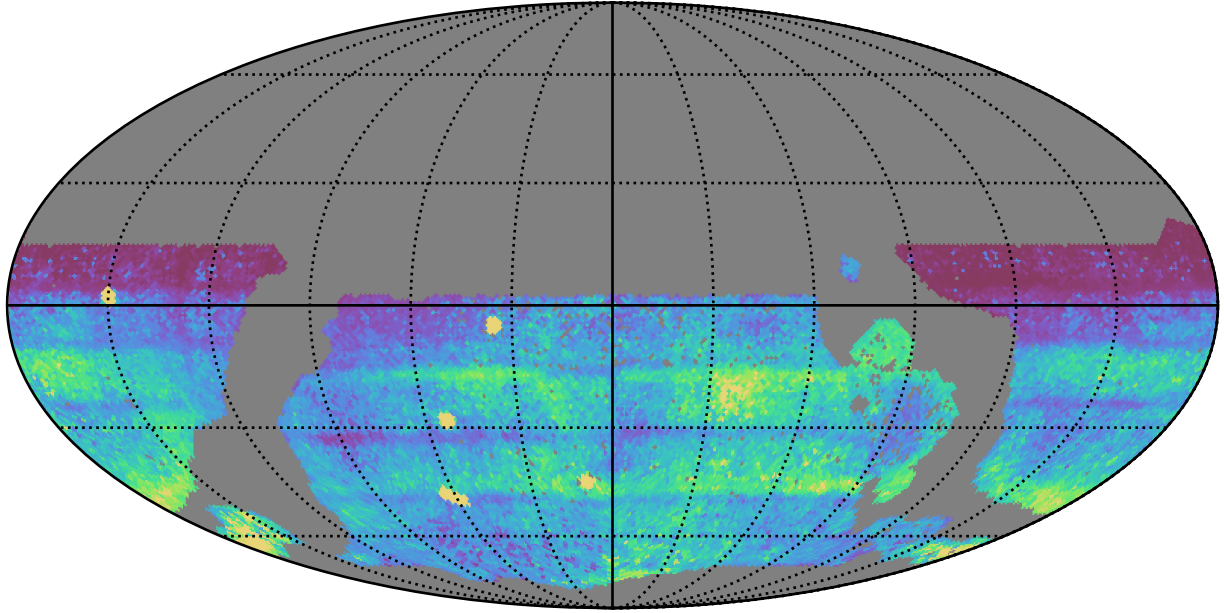
too_combined_s0.8_v3.4_10yrs WFD all bands: 75th Percentile Intranight Timespan
