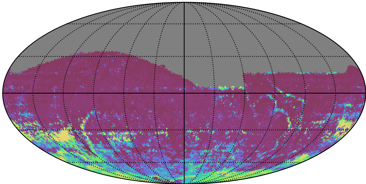
too_combined_s0.8_v3.4_10yrs All sky r band: 75th Percentile Intranight Timespan
