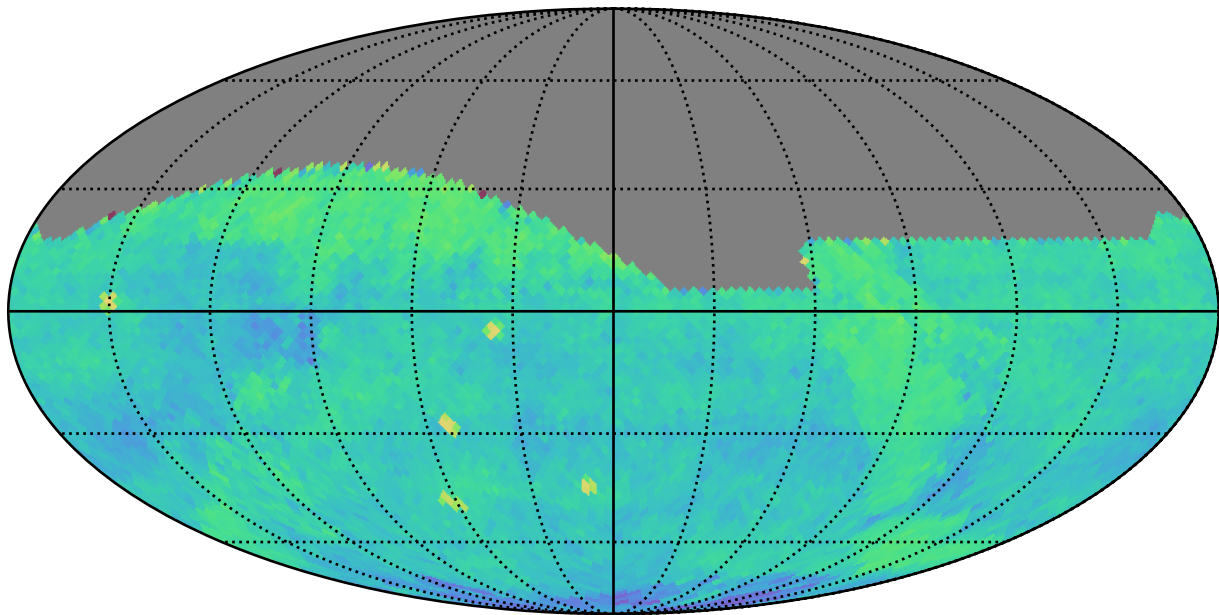
too_combined_s0.8_v3.4_10yrs (g or r or i): PairFraction
