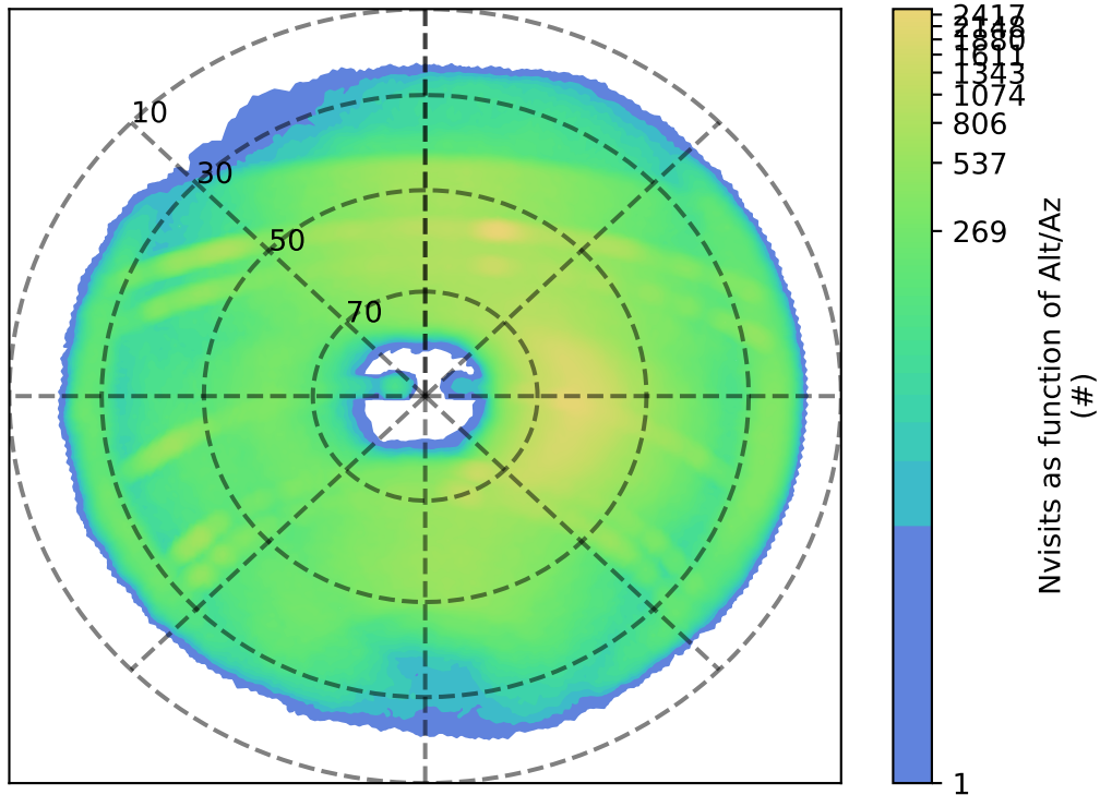
too_combined_s0.8_v3.4_10yrs z: Nvisits as function of Alt/Az
