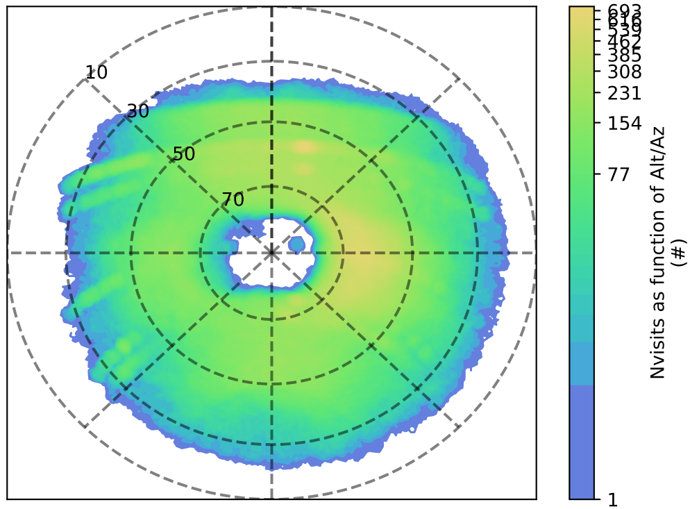
too_combined_s0.8_v3.4_10yrs u: Nvisits as function of Alt/Az
