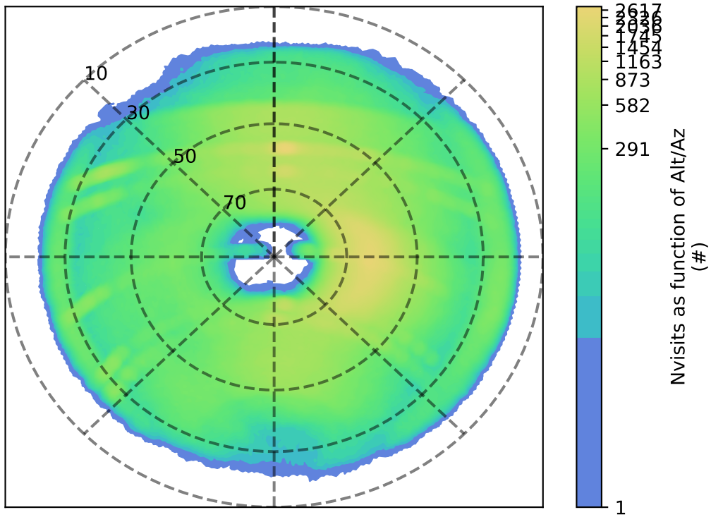
too_combined_s0.8_v3.4_10yrs i: Nvisits as function of Alt/Az
