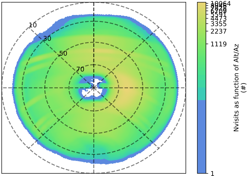
too_combined_s0.8_v3.4_10yrs : Nvisits as function of Alt/Az
