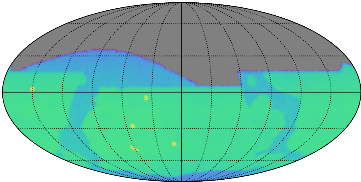
too_combined_s0.8_v3.4_10yrs z: CoaddM5
