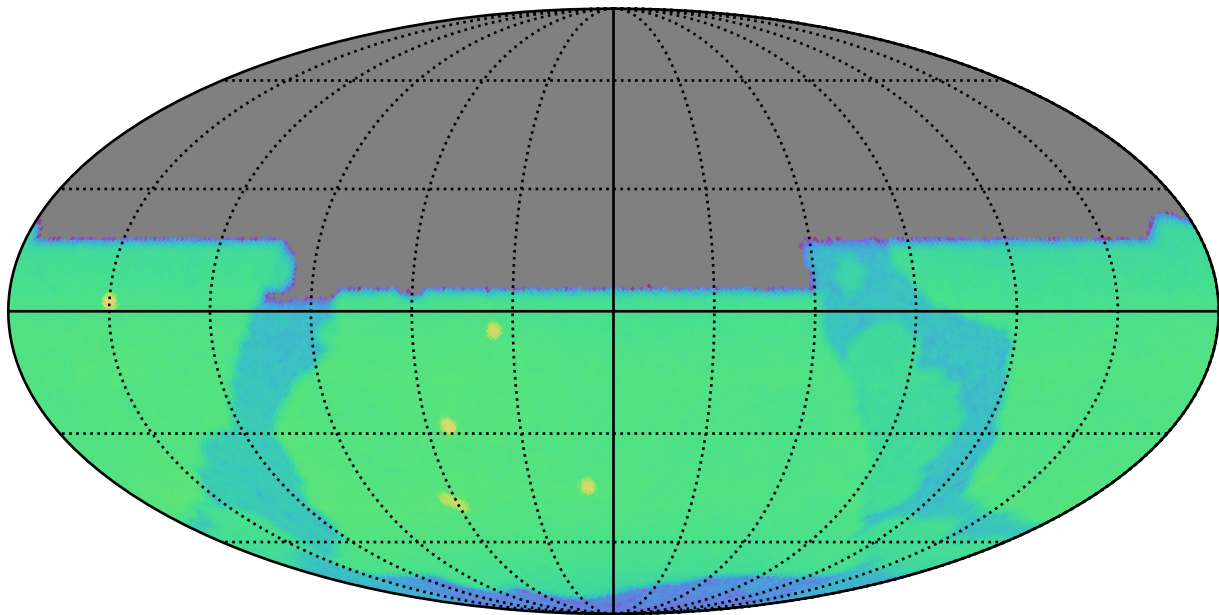
too_combined_s0.8_v3.4_10yrs y: CoaddM5
