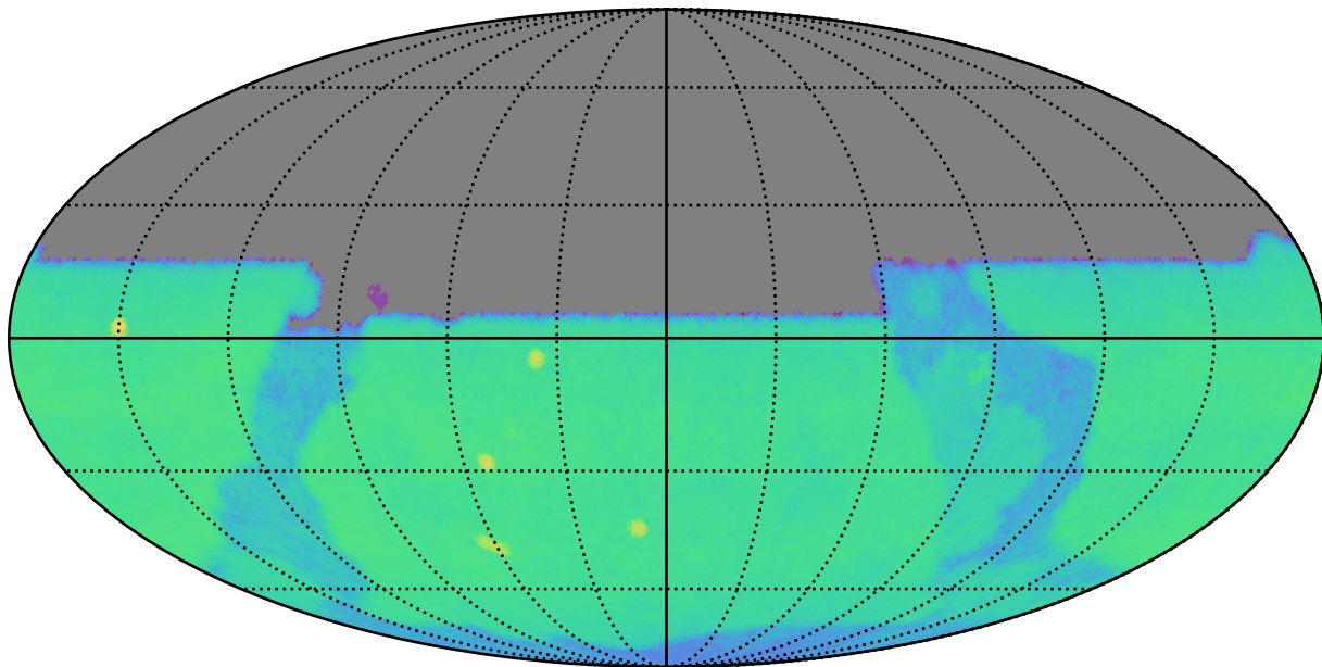
too_combined_s0.8_v3.4_10yrs u: CoaddM5
