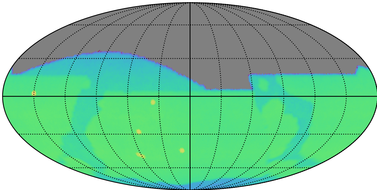
too_combined_s0.8_v3.4_10yrs r: CoaddM5
