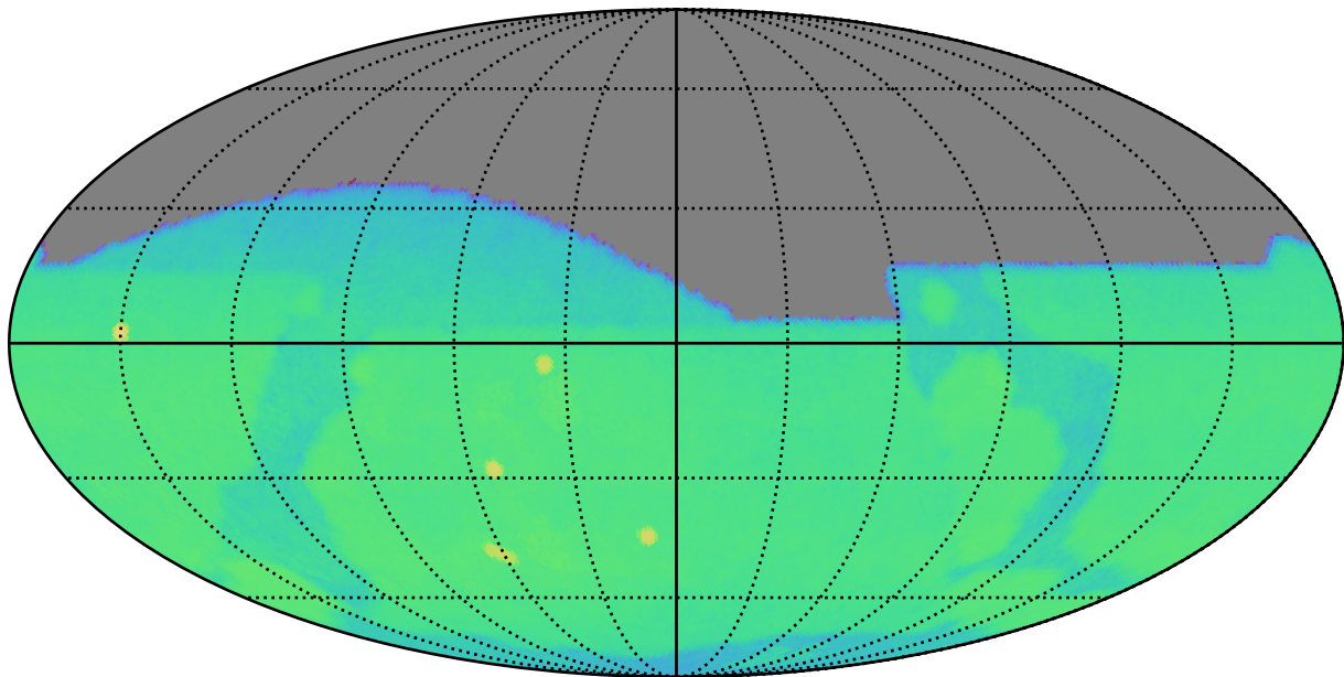
too_combined_s0.8_v3.4_10yrs g: CoaddM5
