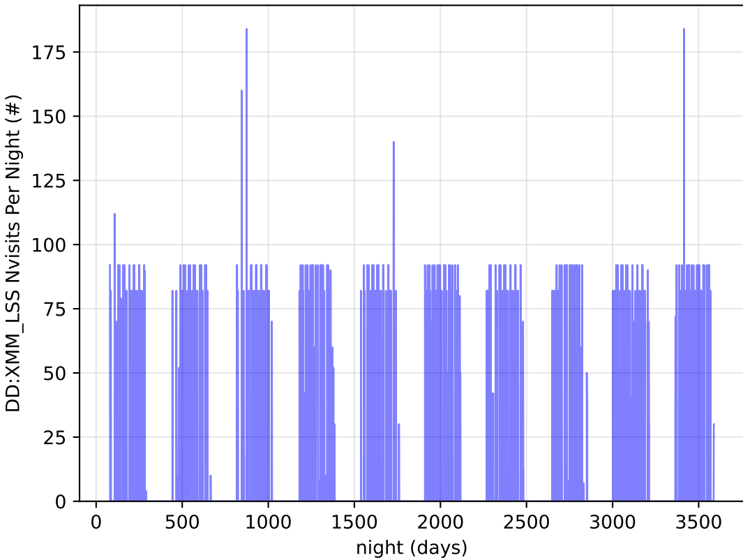
too_combined_s0.8_v3.4_10yrs all bands: DD:XMM_LSS Nvisits Per Night
