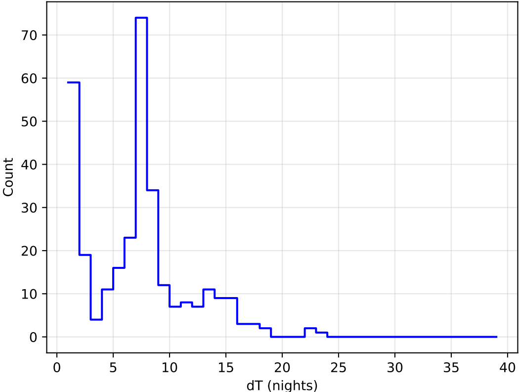
too_combined_s0.8_v3.4_10yrs all bands: DD:XMM_LSS Delta Nights Histogram
