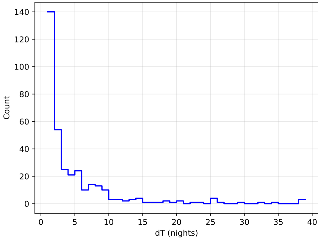
too_combined_s0.8_v3.4_10yrs all bands: DD:WFD Delta Nights Histogram
