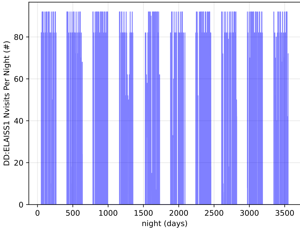
too_combined_s0.8_v3.4_10yrs all bands: DD:ELAISS1 Nvisits Per Night
