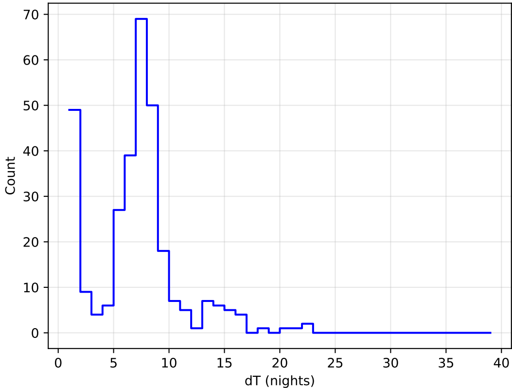
too_combined_s0.8_v3.4_10yrs all bands: DD:ELAISS1 Delta Nights Histogram
