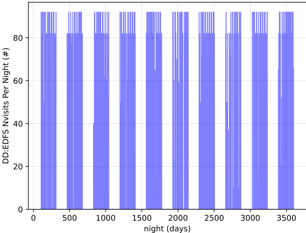
too_combined_s0.8_v3.4_10yrs all bands: DD:EDFS Nvisits Per Night
