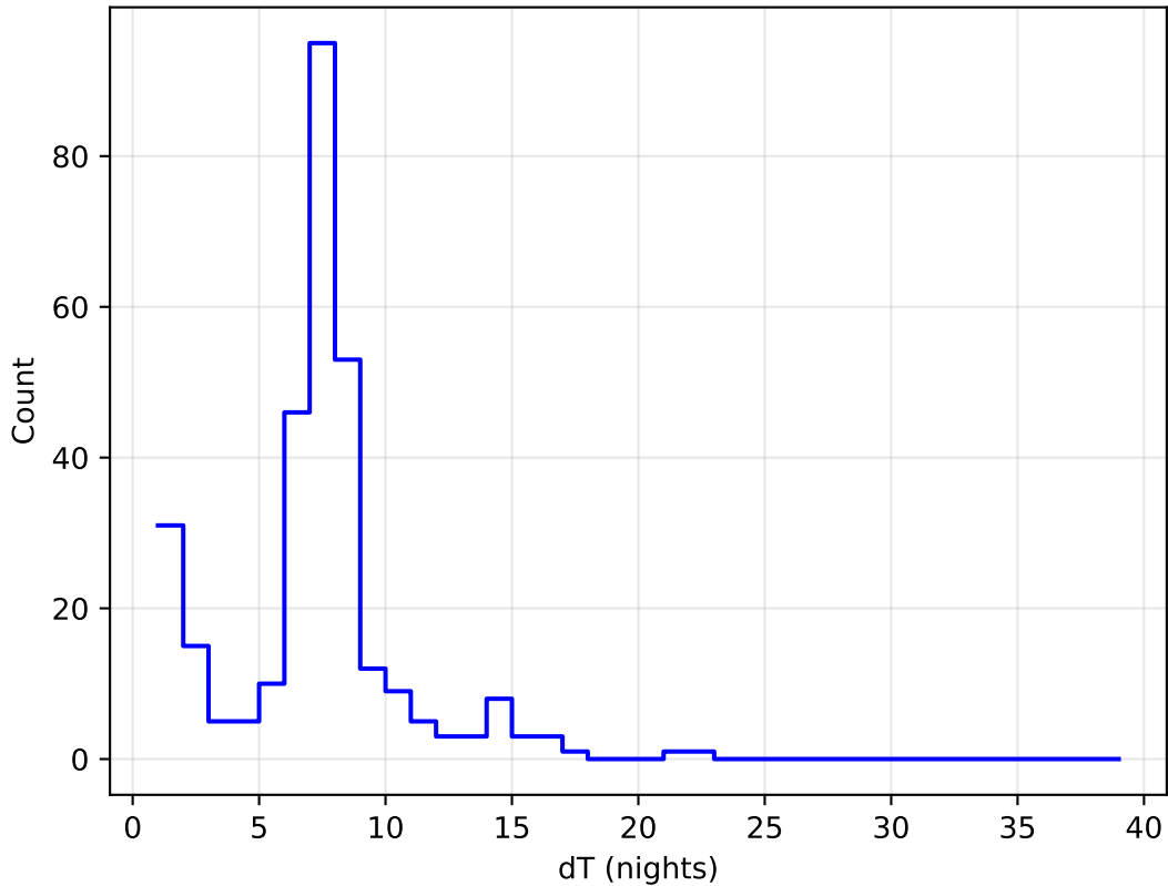
too_combined_s0.8_v3.4_10yrs all bands: DD:EDFS Delta Nights Histogram
