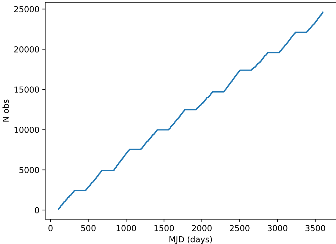
too_combined_s0.8_v3.4_10yrs all bands: DD:EDFS Cumulative NVisits
