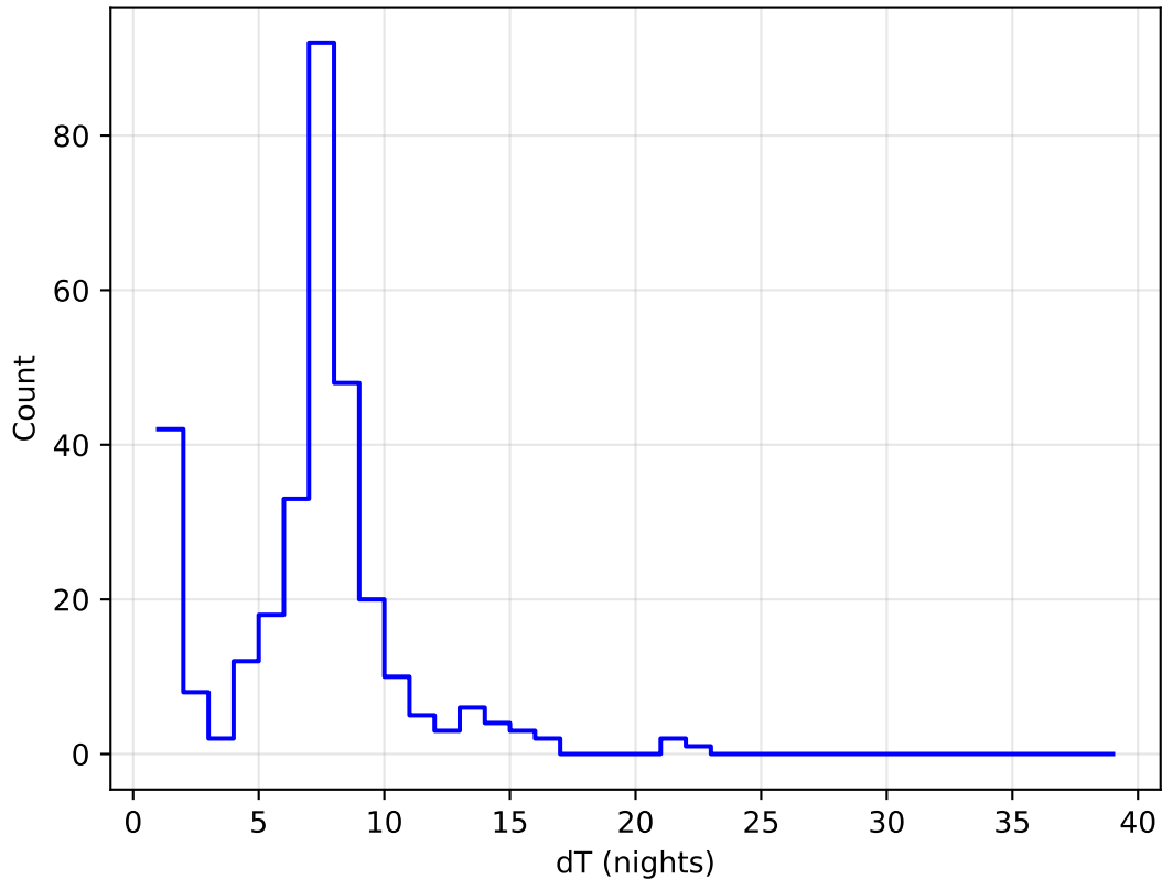
too_combined_s0.8_v3.4_10yrs all bands: DD:ECDFS Delta Nights Histogram
