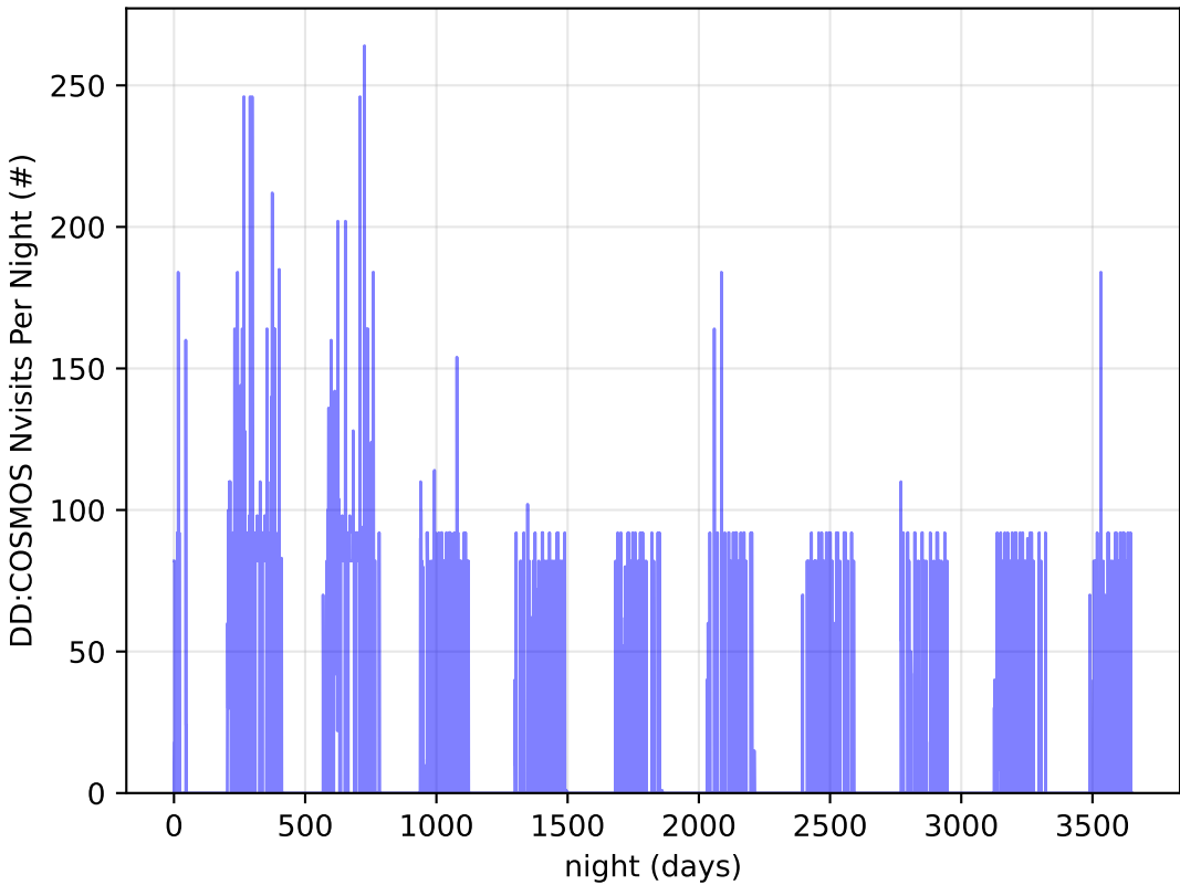
too_combined_s0.8_v3.4_10yrs all bands: DD:COSMOS Nvisits Per Night
