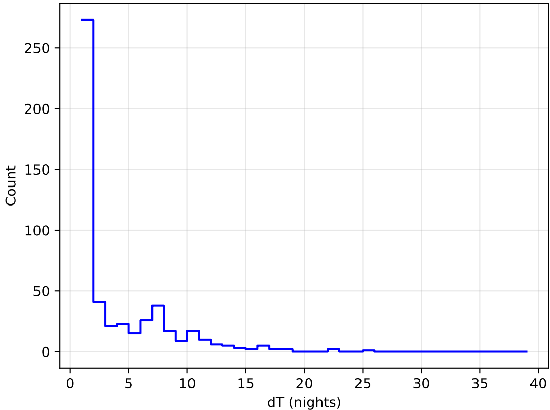
too_combined_s0.8_v3.4_10yrs all bands: DD: COSMOS Delta Nights Histogram
