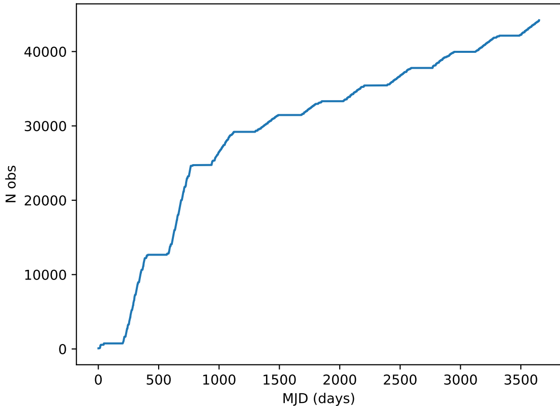
too_combined_s0.8_v3.4_10yrs all bands: DD: COSMOS Cumulative NVisits
