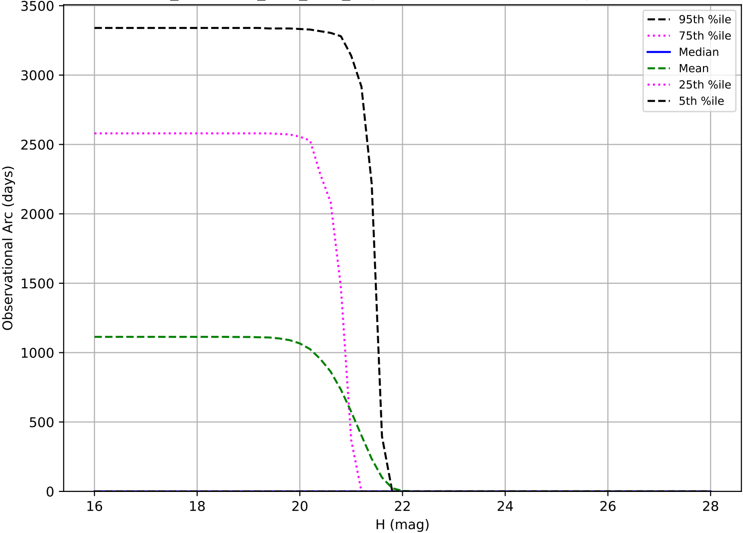
too_combined_s0.5_v3.4_10yrs: Observational Arc Length Vatra
