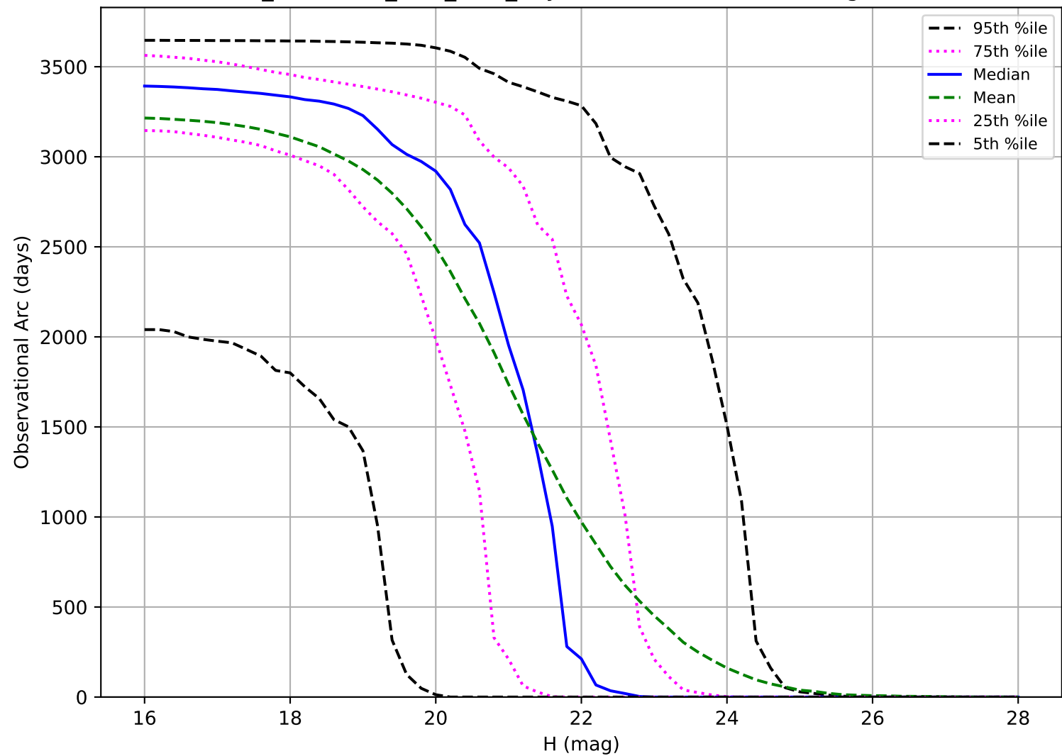
too_combined_s0.5_v3.4_10yrs: Observational Arc Length PHA
