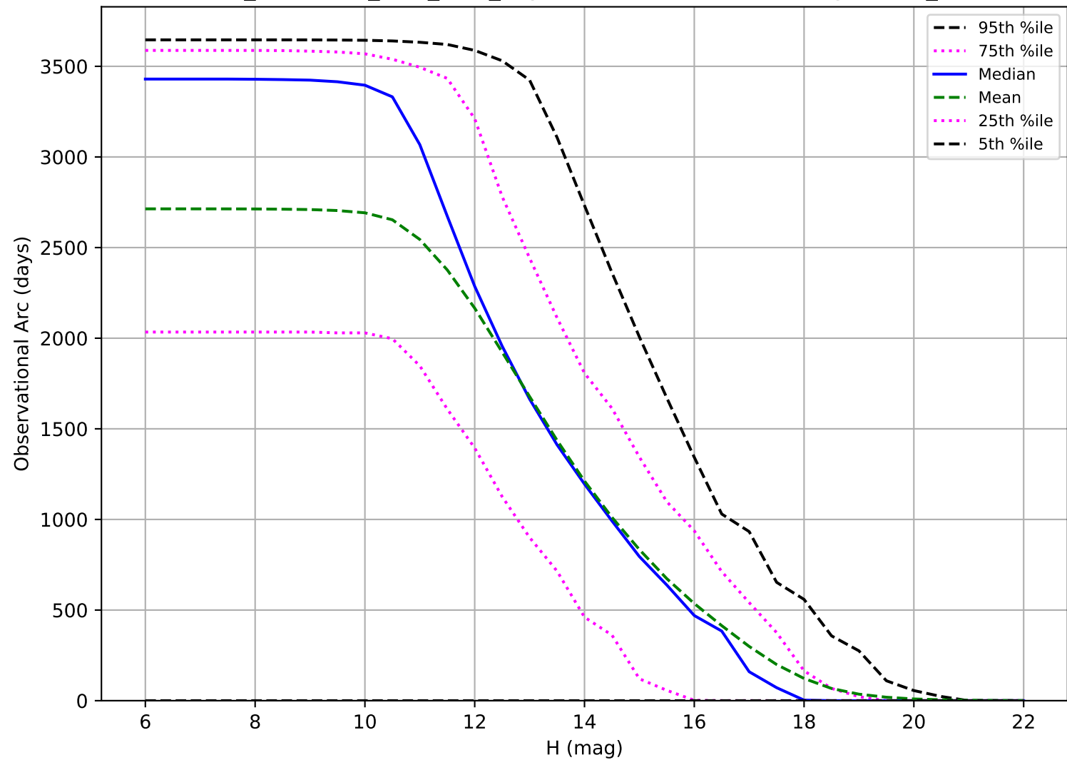
too_combined_s0.5_v3.4_10yrs: Observational Arc Length OCC_r5
