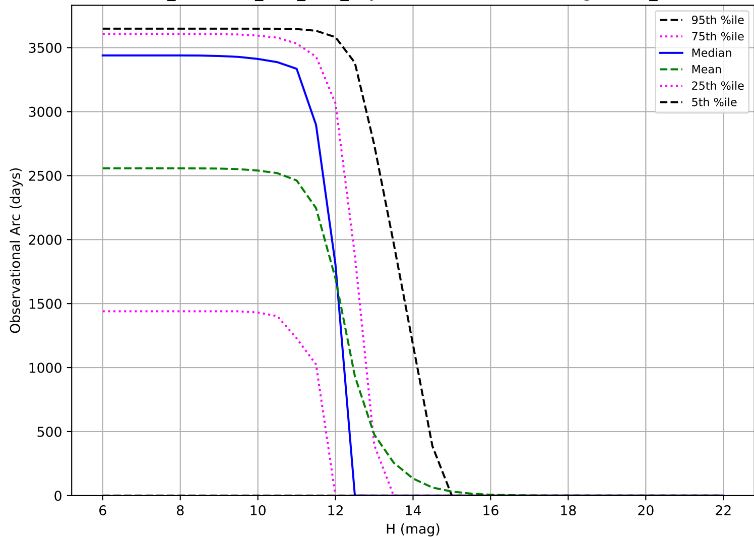
too_combined_s0.5_v3.4_10yrs: Observational Arc Length OCC_r20
