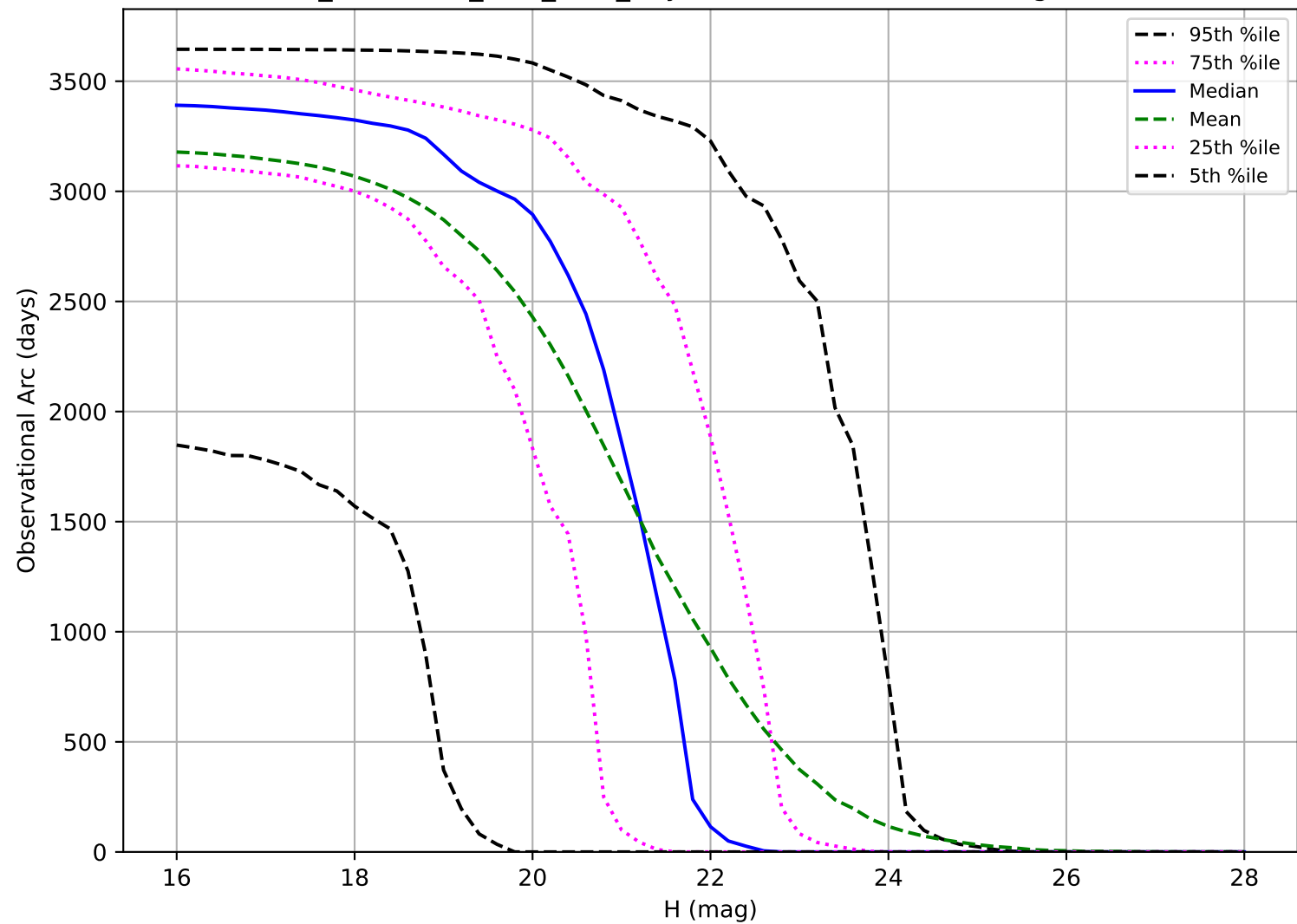
too_combined_s0.5_v3.4_10yrs: Observational Arc Length NEO
