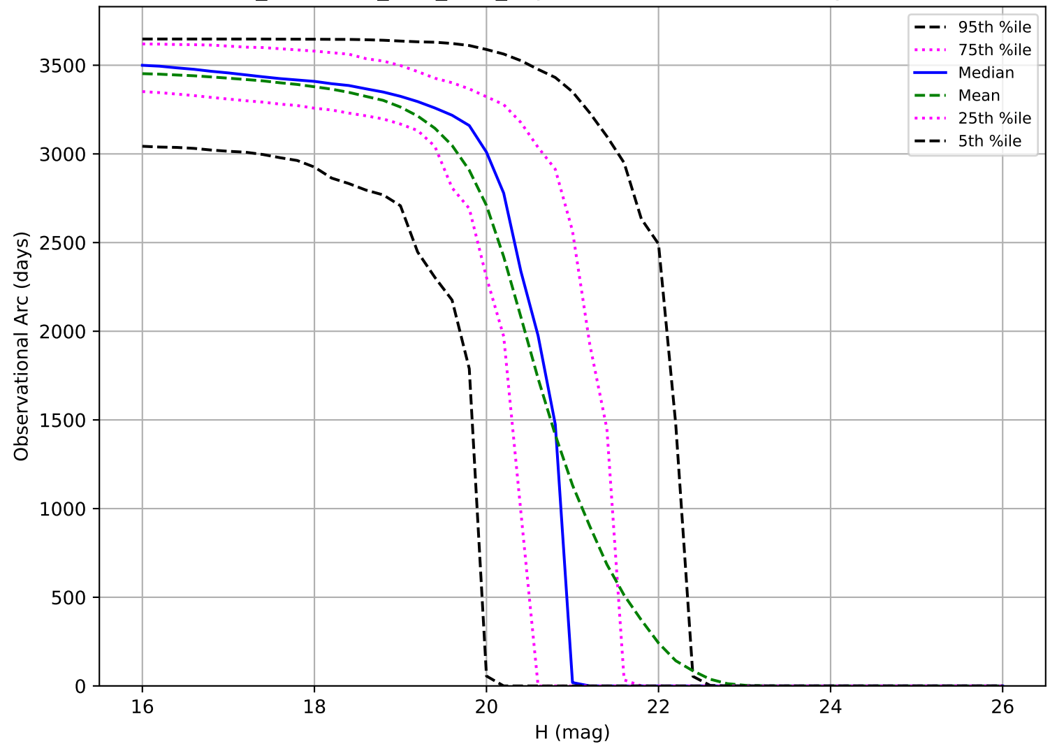
too_combined_s0.5_v3.4_10yrs: Observational Arc Length MBA
