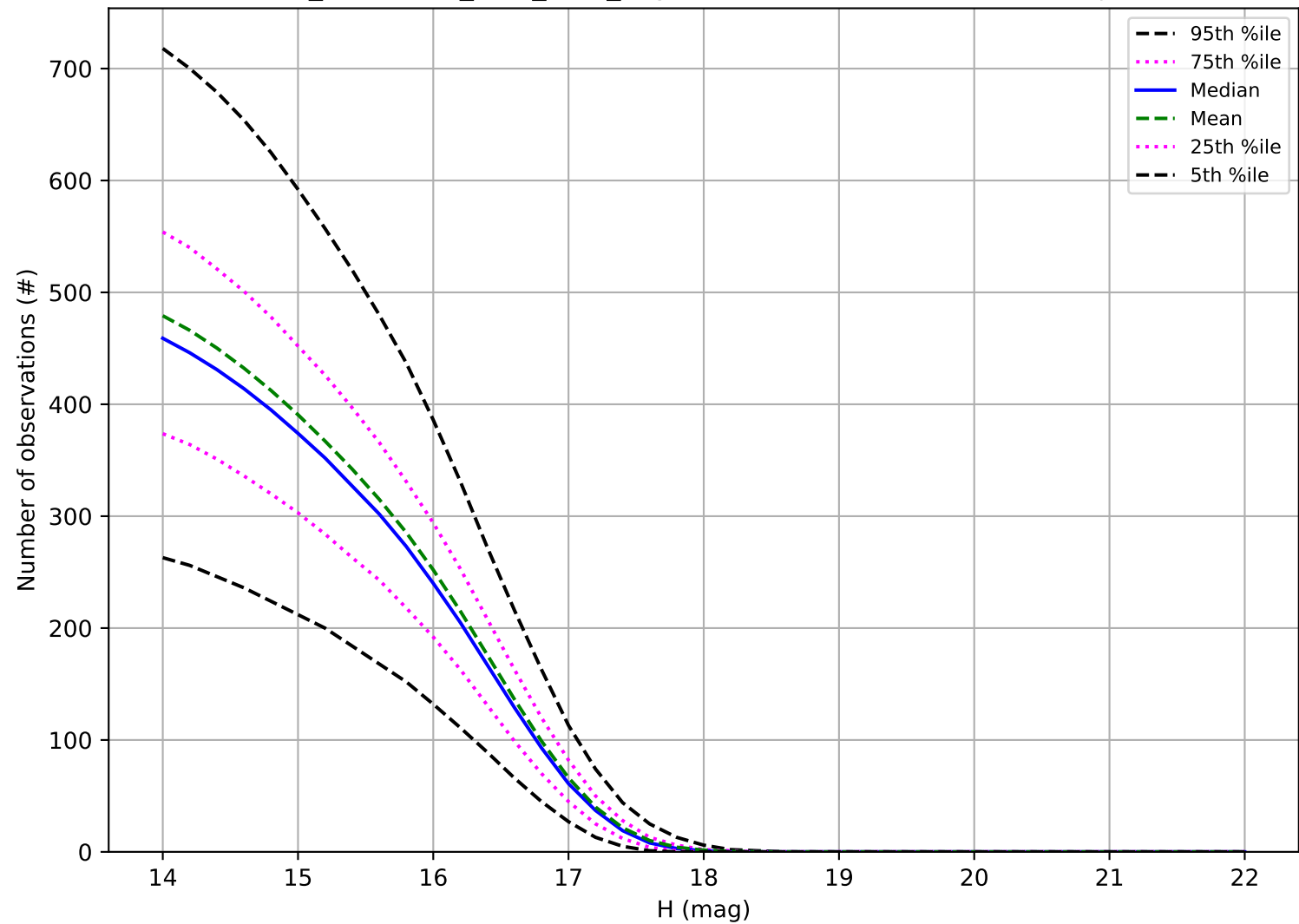
too_combined_s0.5_v3.4_10yrs: Number of observations Trojan
