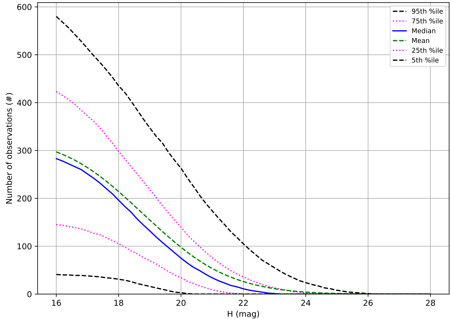
too_combined_s0.5_v3.4_10yrs: Number of observations PHA
