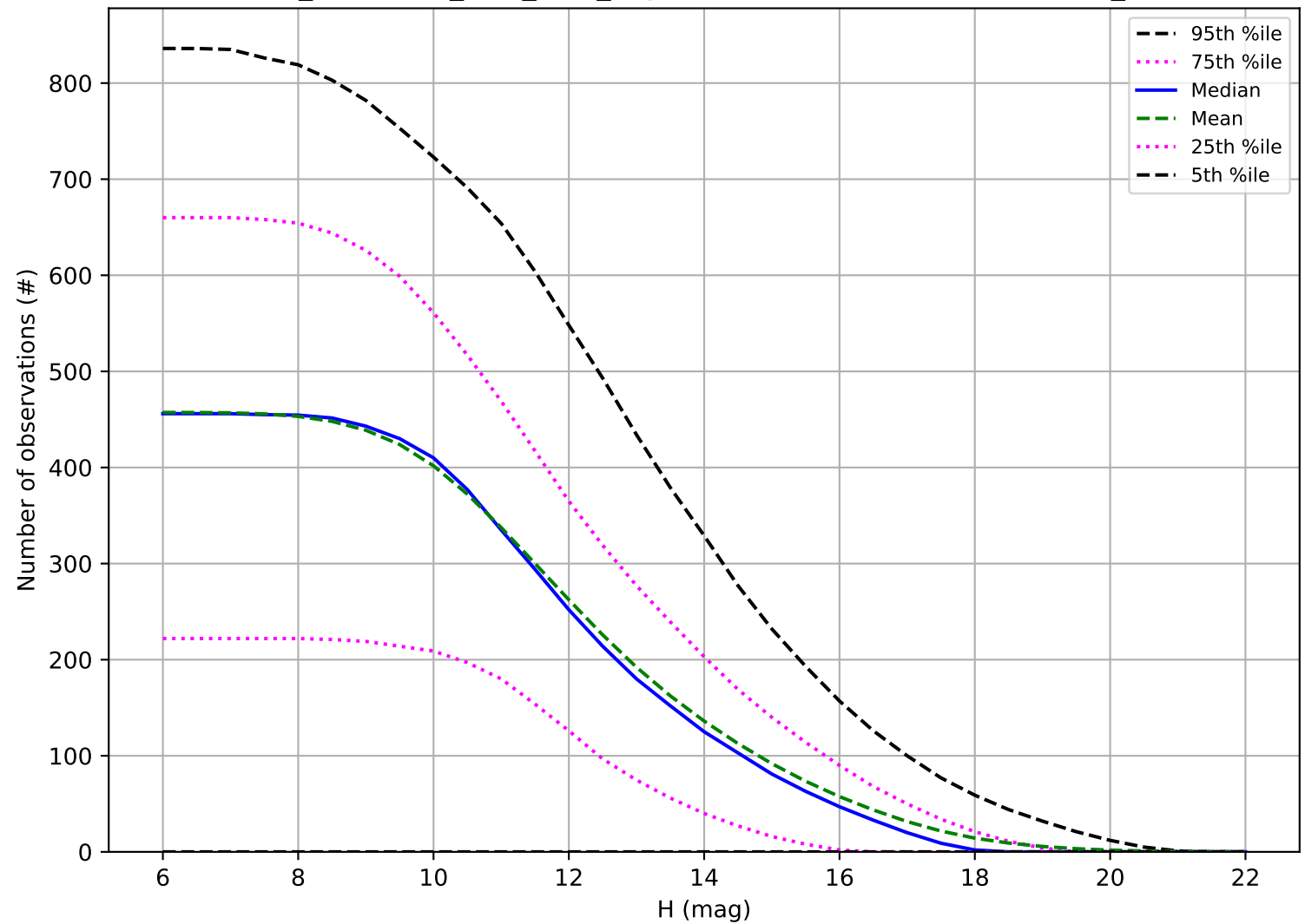
too_combined_s0.5_v3.4_10yrs: Number of observations OCC_r5
