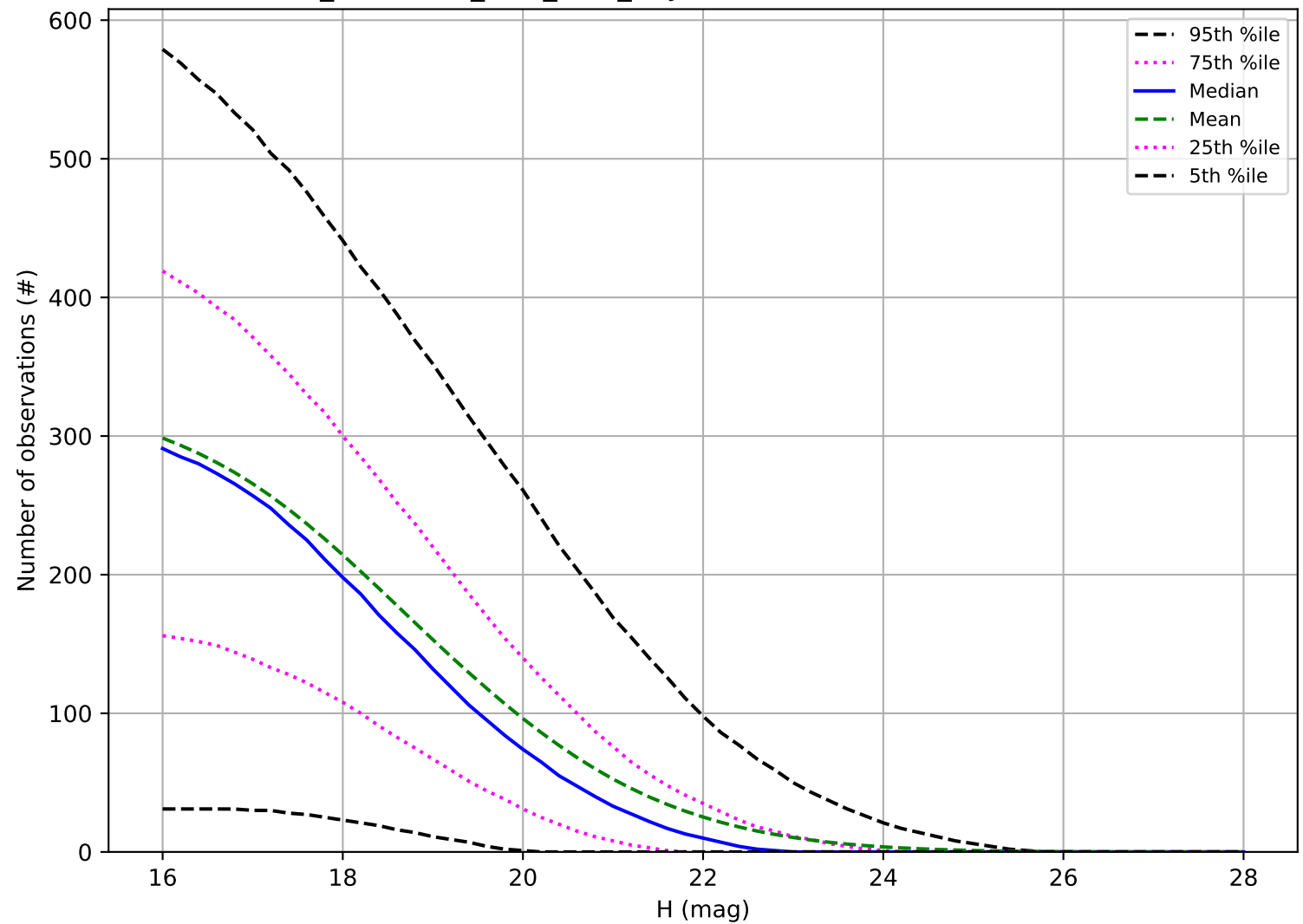
too_combined_s0.5_v3.4_10yrs: Number of observations NEO
