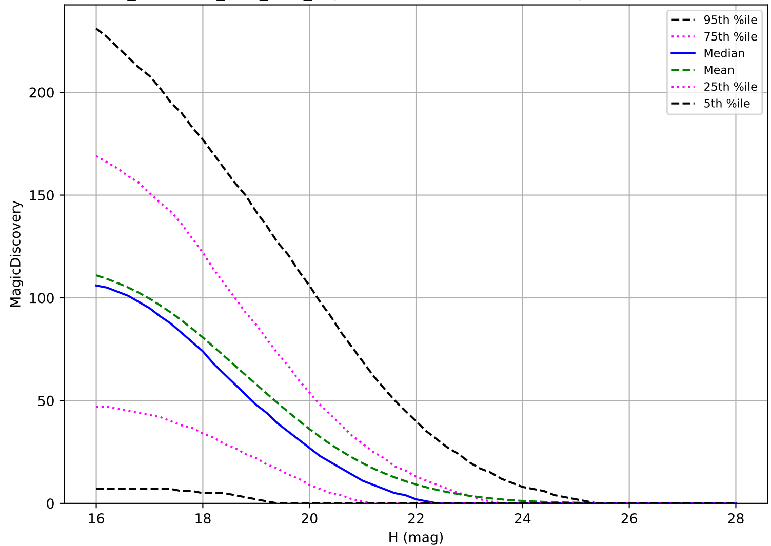
too_combined_s0.5_v3.4_10yrs: PHA 6 detections in 60 nights detection loss
