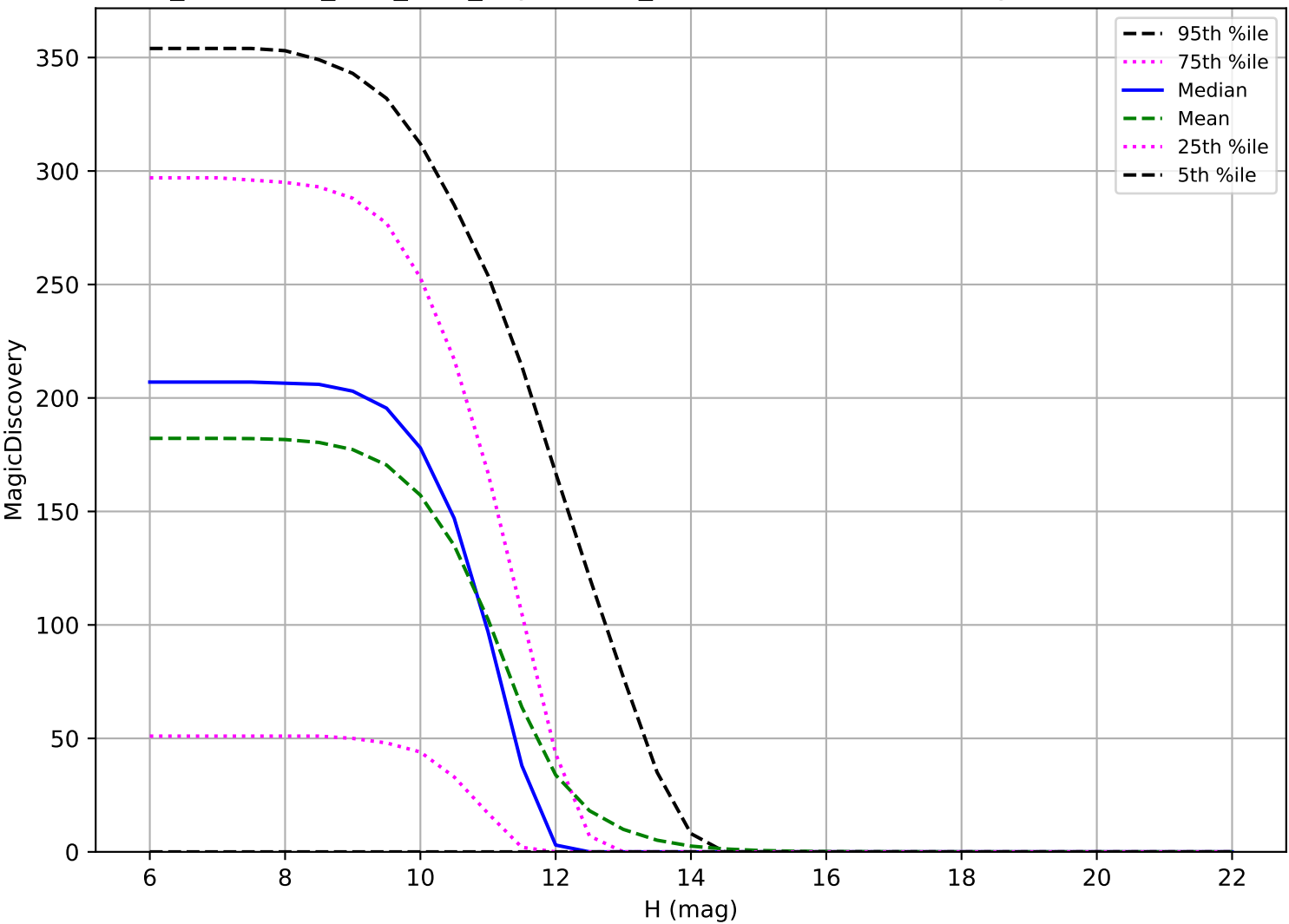
too_combined_s0.5_v3.4_10yrs: OCC_r20 6 detections in 60 nights detection loss
