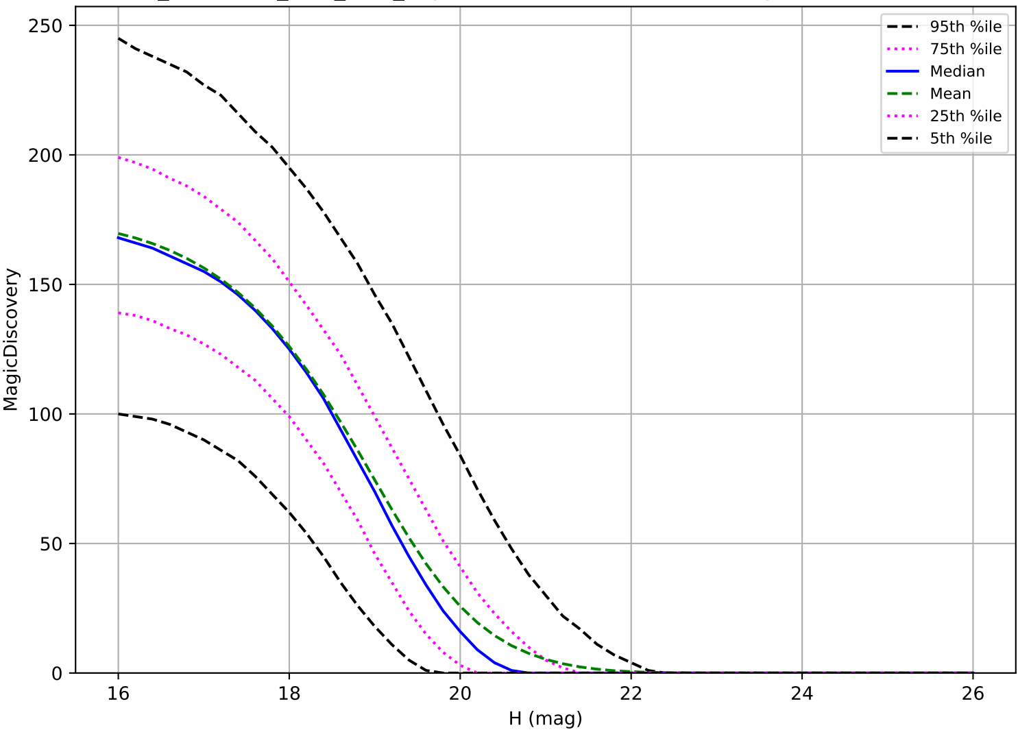
too_combined_s0.5_v3.4_10yrs: MBA 6 detections in 60 nights detection loss
