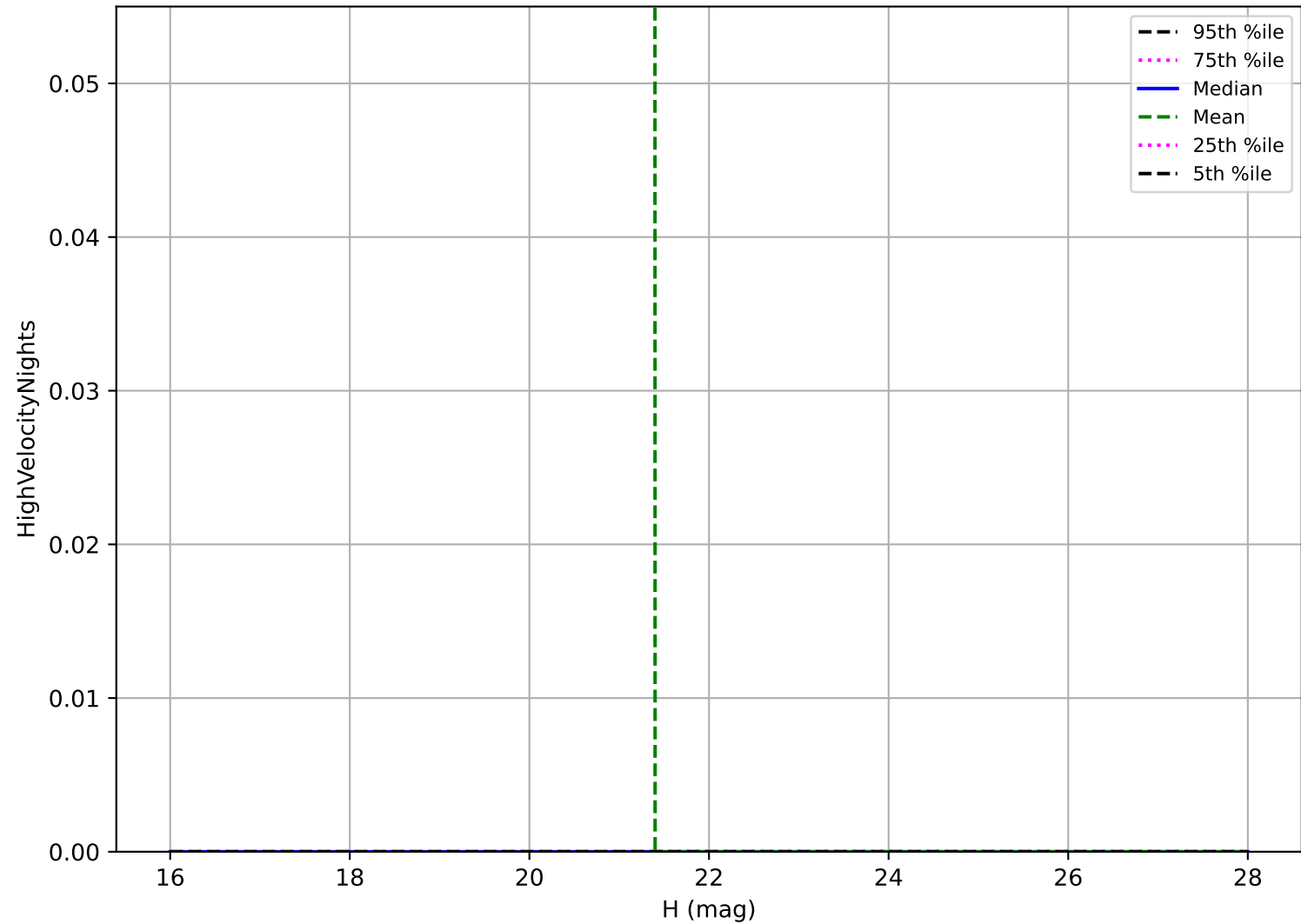
too_combined_s0.5_v3.4_10yrs: Vatira High velocity pair detection loss
