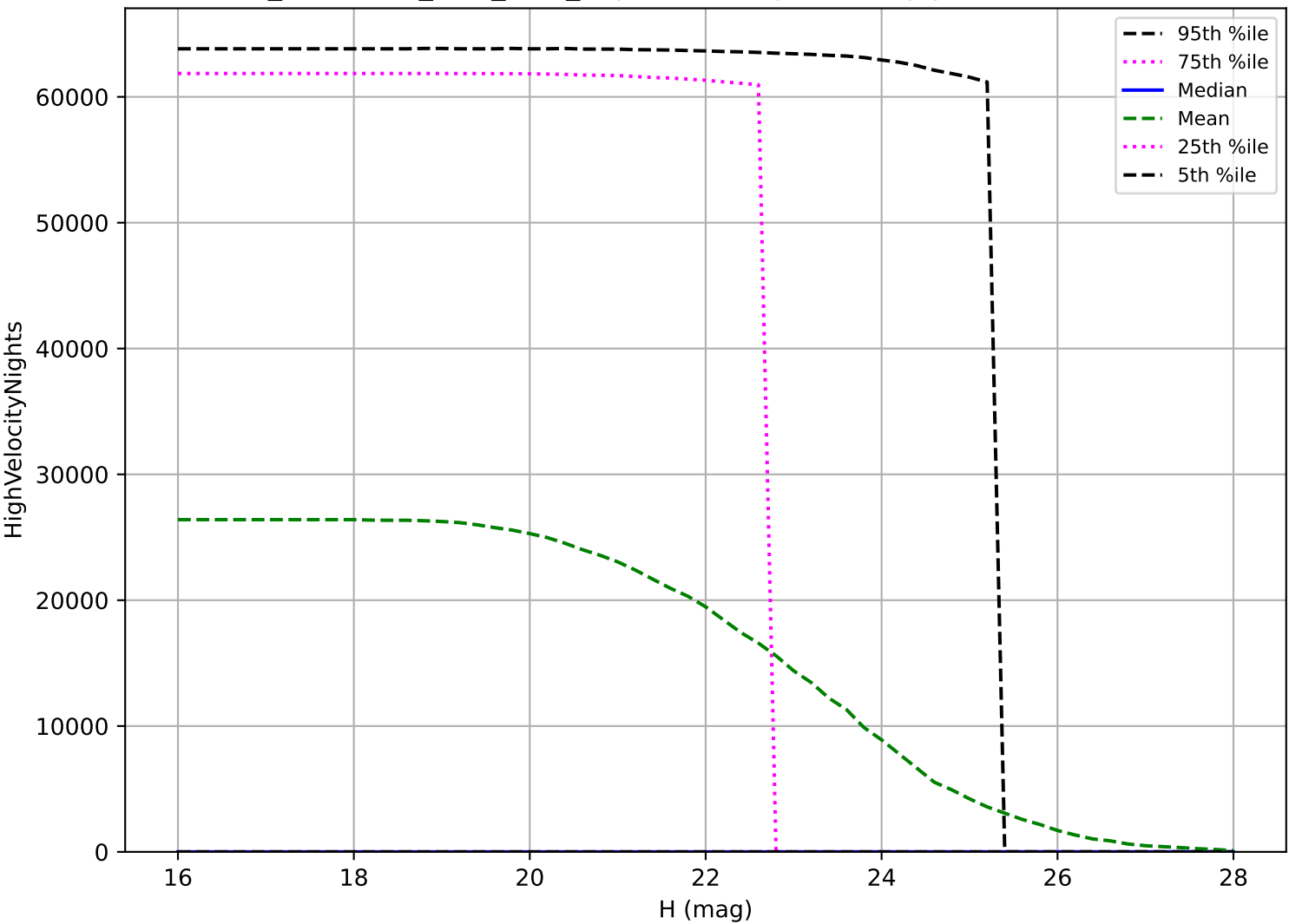
too_combined_s0.5_v3.4_10yrs: PHA High velocity pair detection loss
