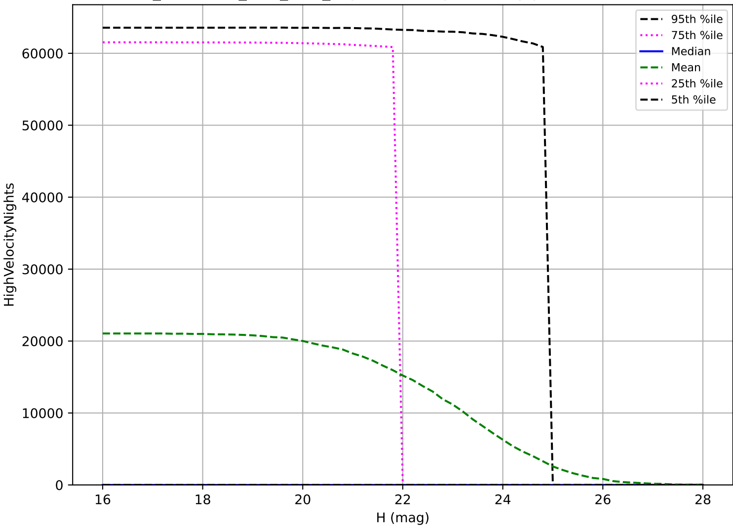
too_combined_s0.5_v3.4_10yrs: NEO High velocity pair detection loss
