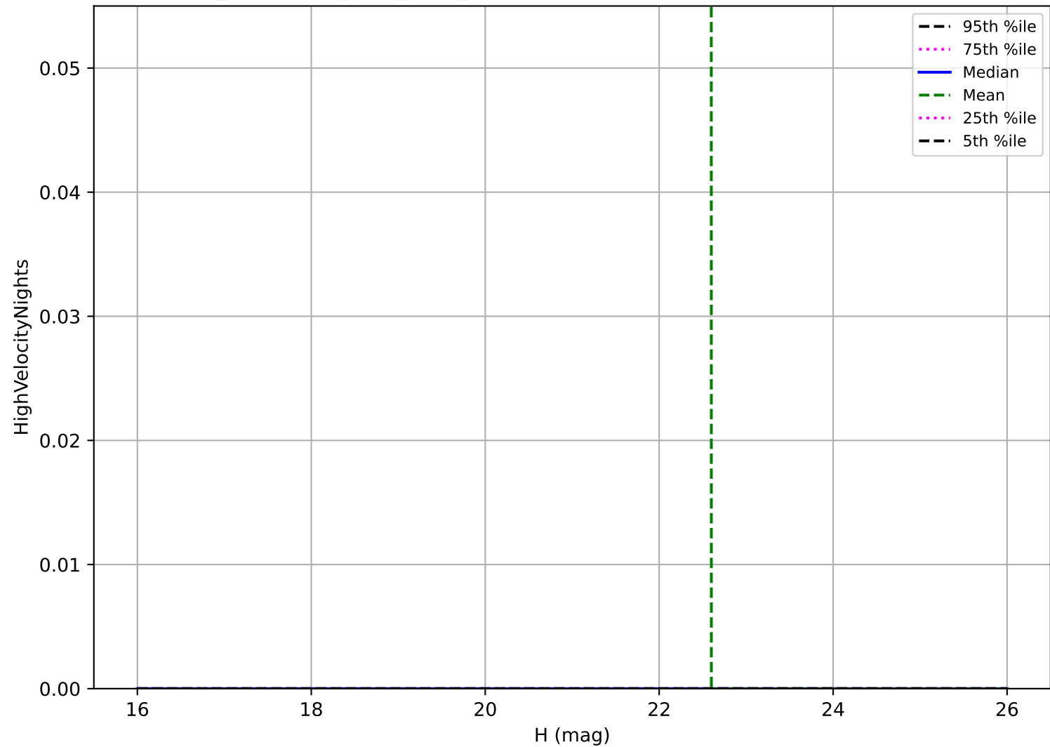
too_combined_s0.5_v3.4_10yrs: MBA High velocity pair detection loss
