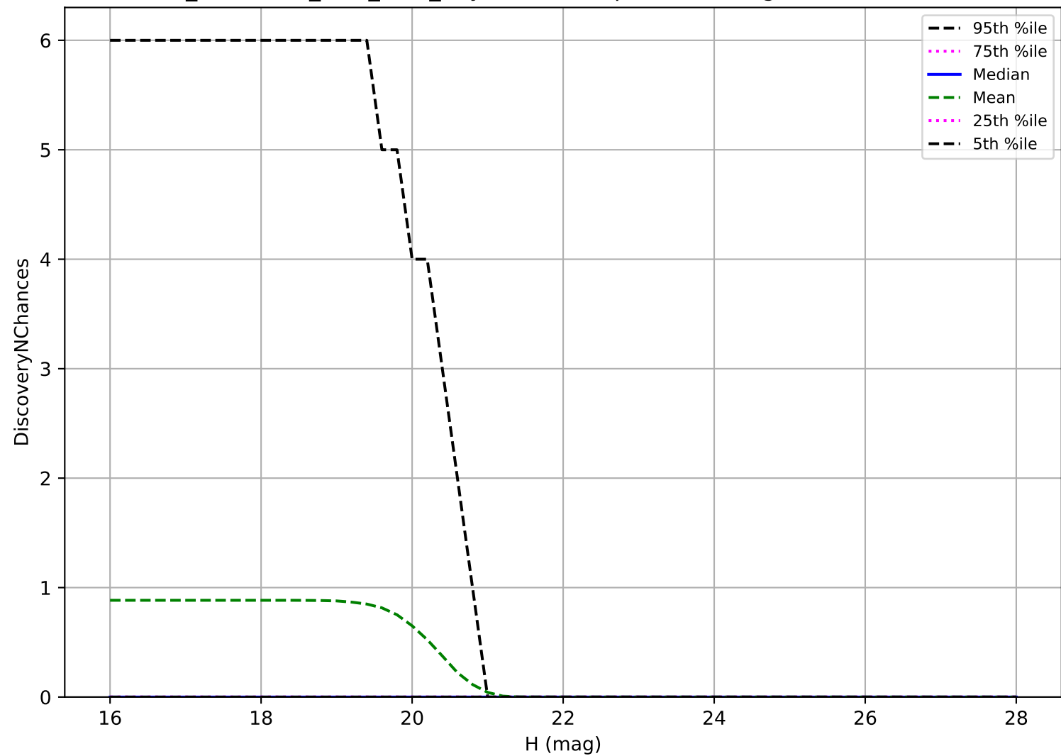
too_combined_s0.5_v3.4_10yrs: Vatira 3 pairs in 15 nights detection loss
