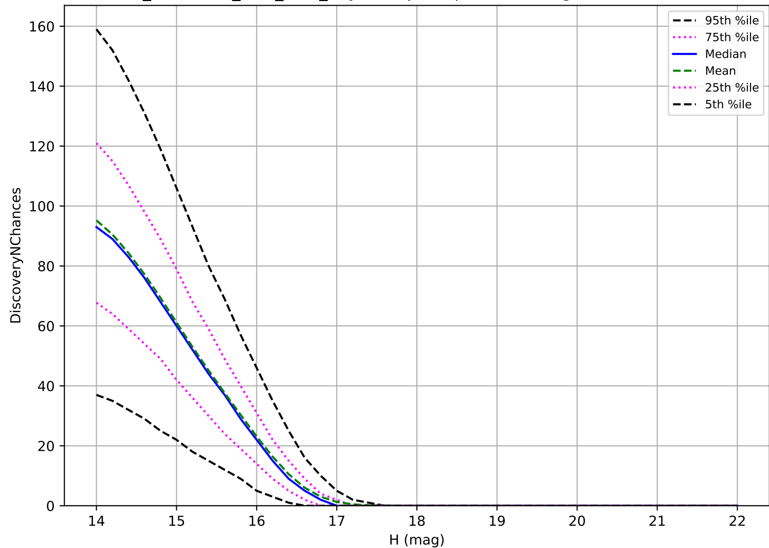
too_combined_s0.5_v3.4_10yrs: Trojan 3 pairs in 15 nights detection loss
