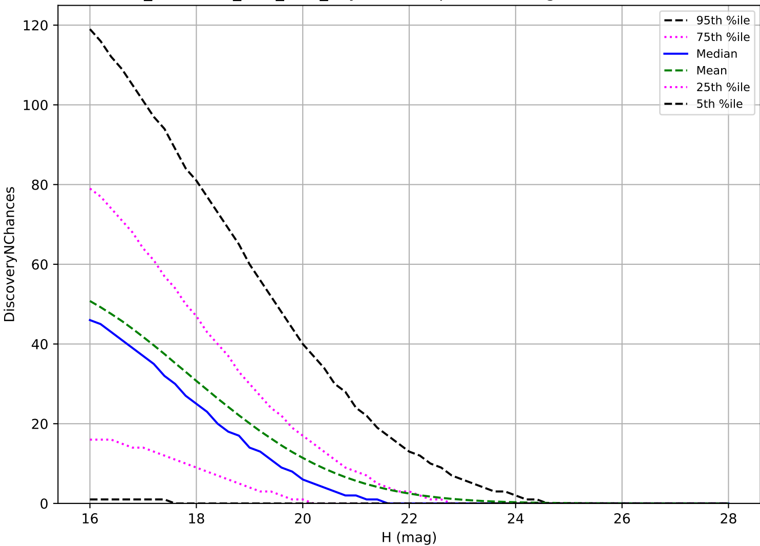
too_combined_s0.5_v3.4_10yrs: PHA 3 pairs in 15 nights detection loss
