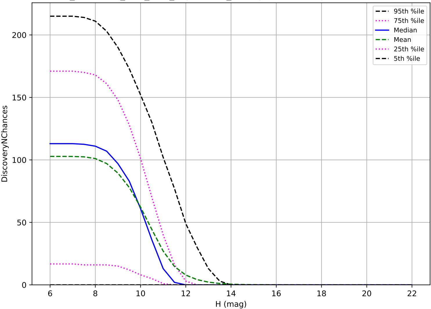
too_combined_s0.5_v3.4_10yrs: OCC_r20 3 pairs in 15 nights detection loss
