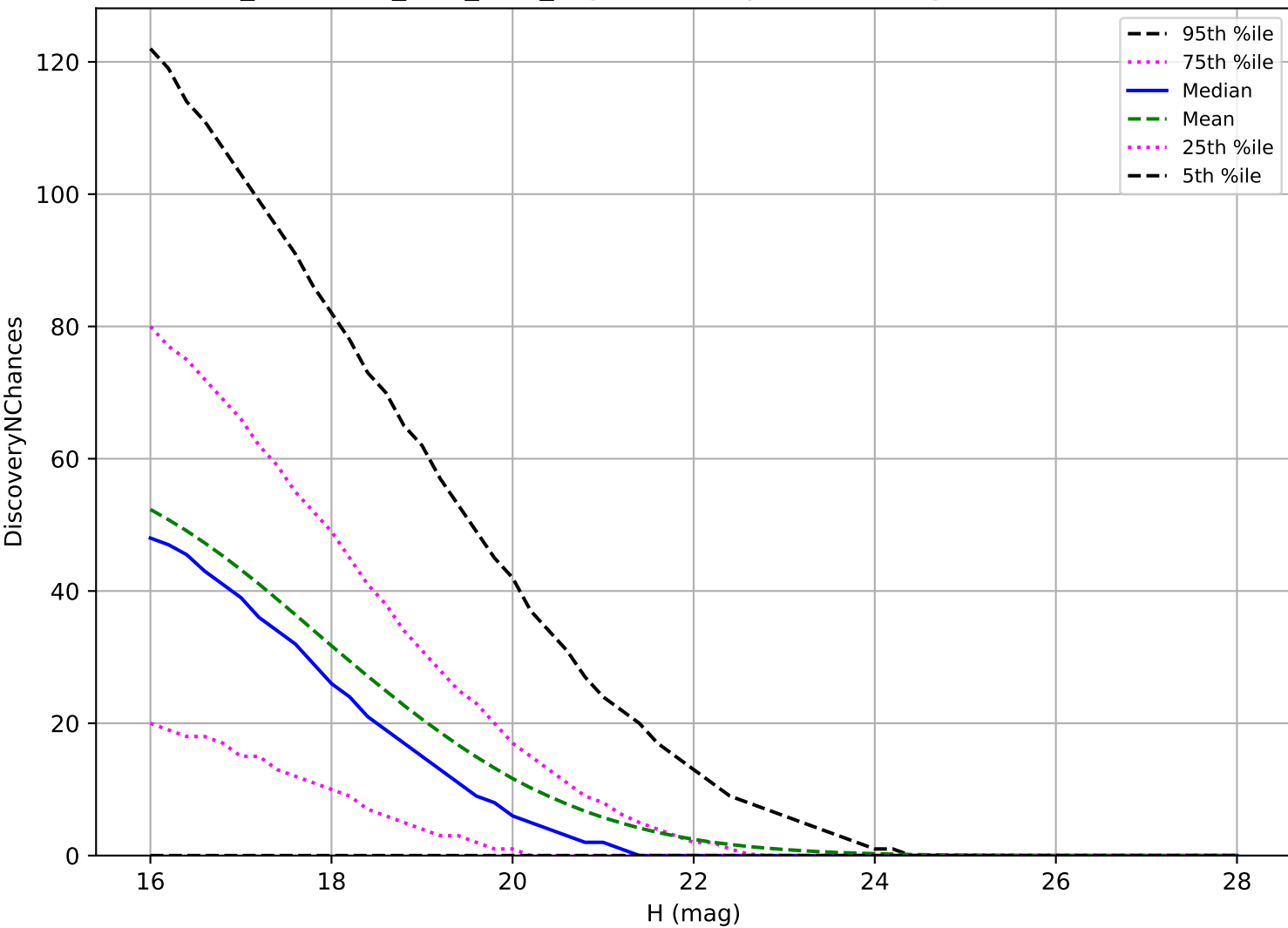
too_combined_s0.5_v3.4_10yrs: NEO 3 pairs in 15 nights detection loss
